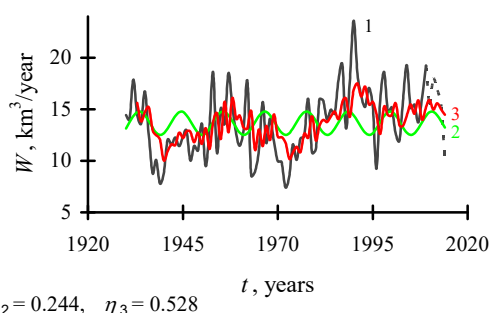
Figure 1. Runoff of local formation of the Novgorod Oblast: 1 – runoff time series, training forecast interval is underlined by the dotted line, 2 – sine with the period of 11 years, 3 – model, formed by the method of Yu.M. Alekhin
